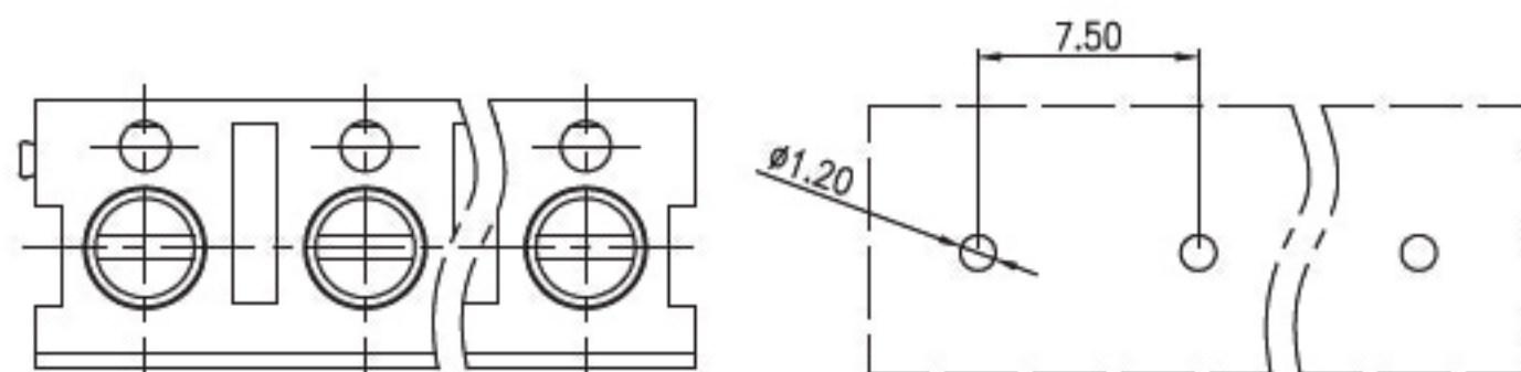
TOP VIEW-LAYOUT
